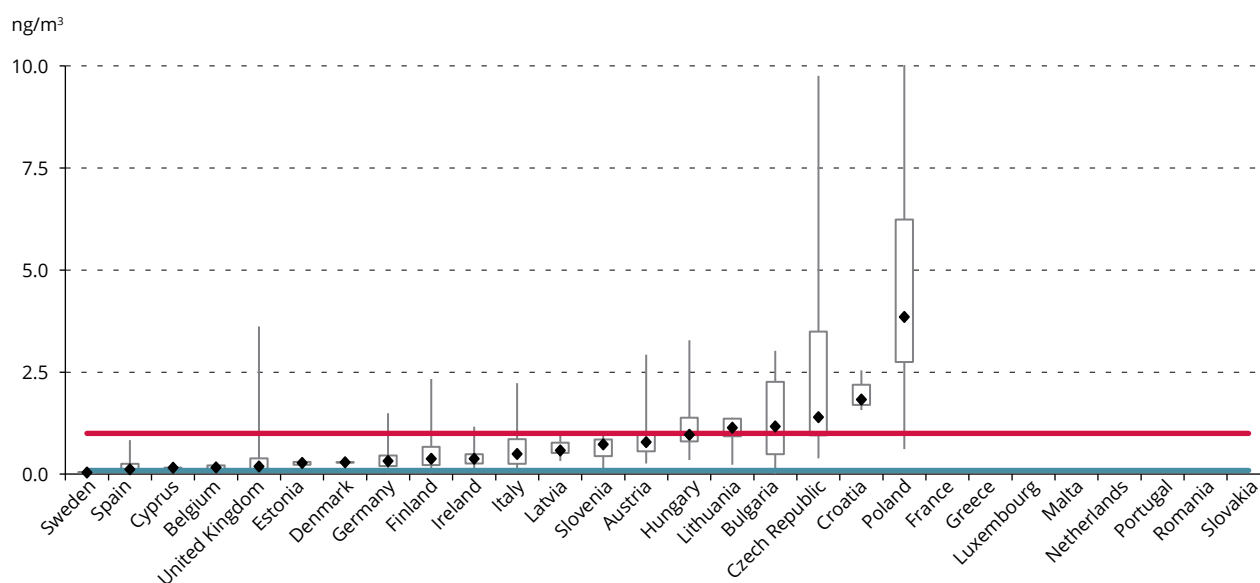
Figure 7.1 BaP concentrations in 2014 in the EU-28
